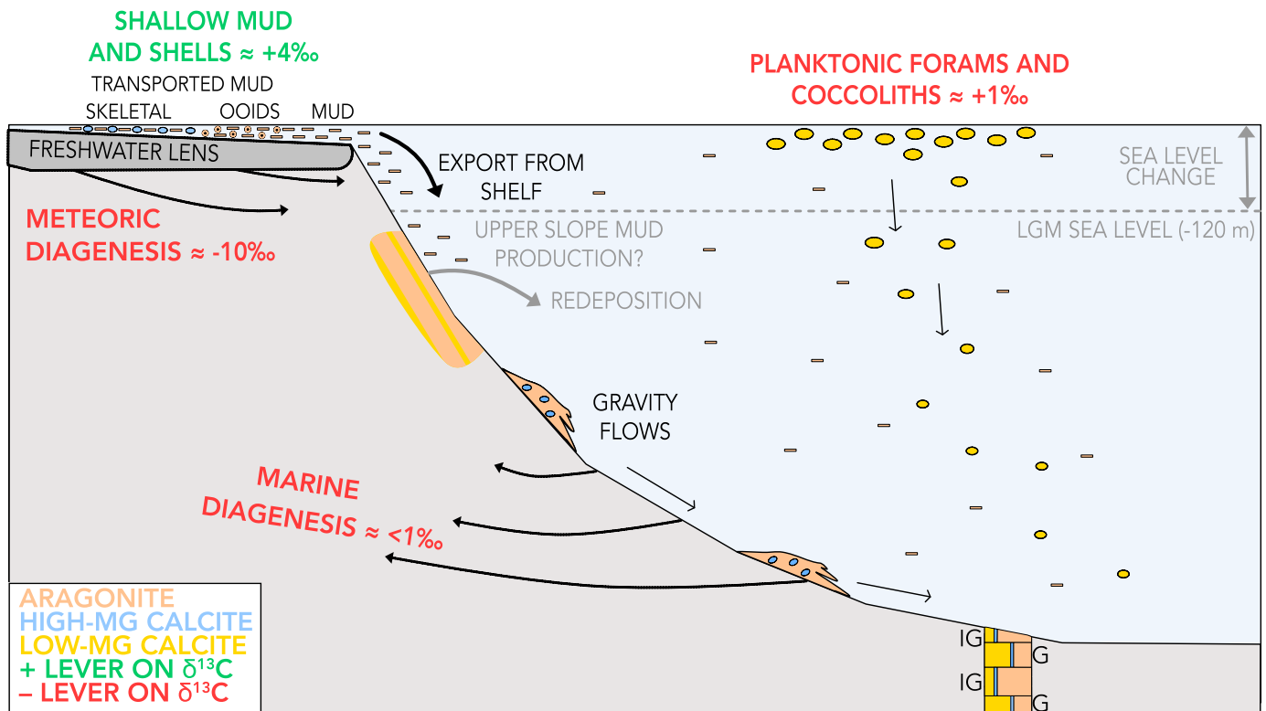
Fig. 1. On the shallow banktop, photosynthesis elevates \delta^{13}\text{C}_{\text{carb}} above the expected value for carbonate precipitated in equilibrium with open-ocean DIC (Geyman and Maloof, 2019). Bahamian banktop carbonate primarily is aragonite with some high-magnesium calcite (HMC) (Swart et al., 2009), while pelagic planktonic forams and coccoliths produced in the mixed layer of the open ocean are composed of low-magnesium calcite (LMC). Exported banktop carbonate raises both the \delta^{13}\text{C} and aragonite fraction of slope carbonate compared to background pelagic sedimentation (Swart and Eberli, 2005). When sea level falls below the platform edge during glacial sea level lowstands, aragonite input is reduced and the fraction of pelagic LMC increases. More limited aragonite mud production likely persists on the upper slopes (Geyman et al., 2022), and older sediment also may be redeposited through winnowing or as gravity flows. While sea level is low, banktop carbonate on the subaerially exposed shelf is cemented and altered by meteoric waters while the periplatformal slope remains submerged. On longer timescales, metastable aragonite and HMC recrystallize to LMC during early marine diagenesis at the seafloor (Higgins et al., 2018).
