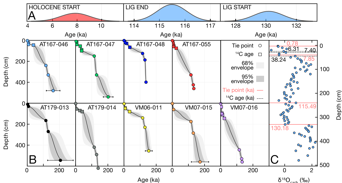
Fig. 4. A) Probability distributions for the timing of the Holocene and the LIG based on dated corals and mangrove peat horizons in the literature (see supplementary material, section 1.9). B) MCMC age-depth models for 9 aligned cores plotted with 68% and 95% confidence envelopes. Tie points and ^{14}\text{C} ages are plotted with 2\sigma uncertainty. C) Example tie point identification for core AT167-046.
