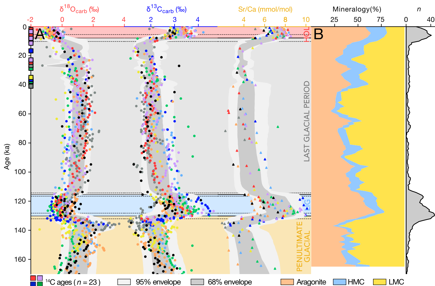
Fig. 5. A) \delta^{18}\text{O}_{\text{carb}} , \delta^{13}\text{C}_{\text{carb}} , and Sr/Ca stratigraphies for 9 periplatform cores aligned using our MCMC age models, which are based only on tie points in \delta^{18}\text{O}_{\text{carb}} and ^{14}\text{C} age constraints. Colors correspond to individual cores as in Fig. 2. Data are plotted by median posterior age, and confidence envelopes are calculated using composite MCMC paths interpolated to a 1 kyr grid. ^{14}\text{C} age constraints (in calendar years B.P.) are plotted on the y-axis. B) Stack of periplatform core mineralogy. Mineralogy stratigraphies for individual cores are in Figs. S32 and S33. In B, each point represents the mean of at least n = 3 samples in a sliding 5 kyr window, with a mean sample size of n = 10.7 . To the right, we show the number of samples within this sliding window.
