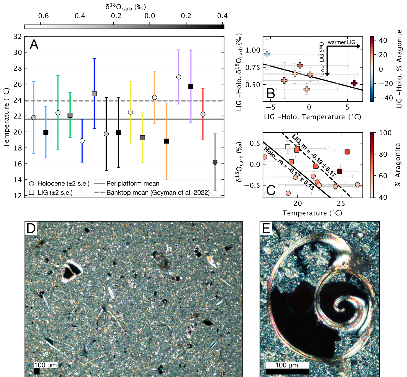
Fig. 8. A) Clumped-isotope temperatures for Holocene and LIG periplatform core samples. Marker grayscale tracks sediment \delta^{18}\text{O} , while error bar colors correspond to individual cores as in Fig. 2. B) For cores with both Holocene and LIG clumped-isotope temperatures, we examine LIG-Holocene differences in temperature, \delta^{18}\text{O}_{\text{carb}} , and aragonite content. C) Least squares regressions through Holocene and LIG \delta^{18}\text{O}_{\text{carb}} and temperature data. Note that we do not plot the diagenetically altered pre-LIG sample that yielded a temperature of 7.0 \pm 2.0^\circ\text{C} (1 s.e.). D) Example of a typical interglacial wackestone under cross-polarized light. This sample (VM06011-210) is from the LIG, and has a clumped-isotope temperature of 19.3 \pm 1.6^\circ\text{C} (1 s.e.). A point count ( n = 500 ) of this sample reveals 81% carbonate mud, 13% fine skeletal fragments, and 6% larger shell fragments that include gastropods, foraminifera, bivalves, and corals. We observe no cements on the >10 micron scale. E) A well-preserved gastropod from LIG sample AT167048-168, which has a clumped-isotope temperature of 24.8 \pm 2.2^\circ\text{C} (1 s.e.). The shell is partly filled with sediment and shows no evidence of cement growth. Scale bars are 100 microns.
