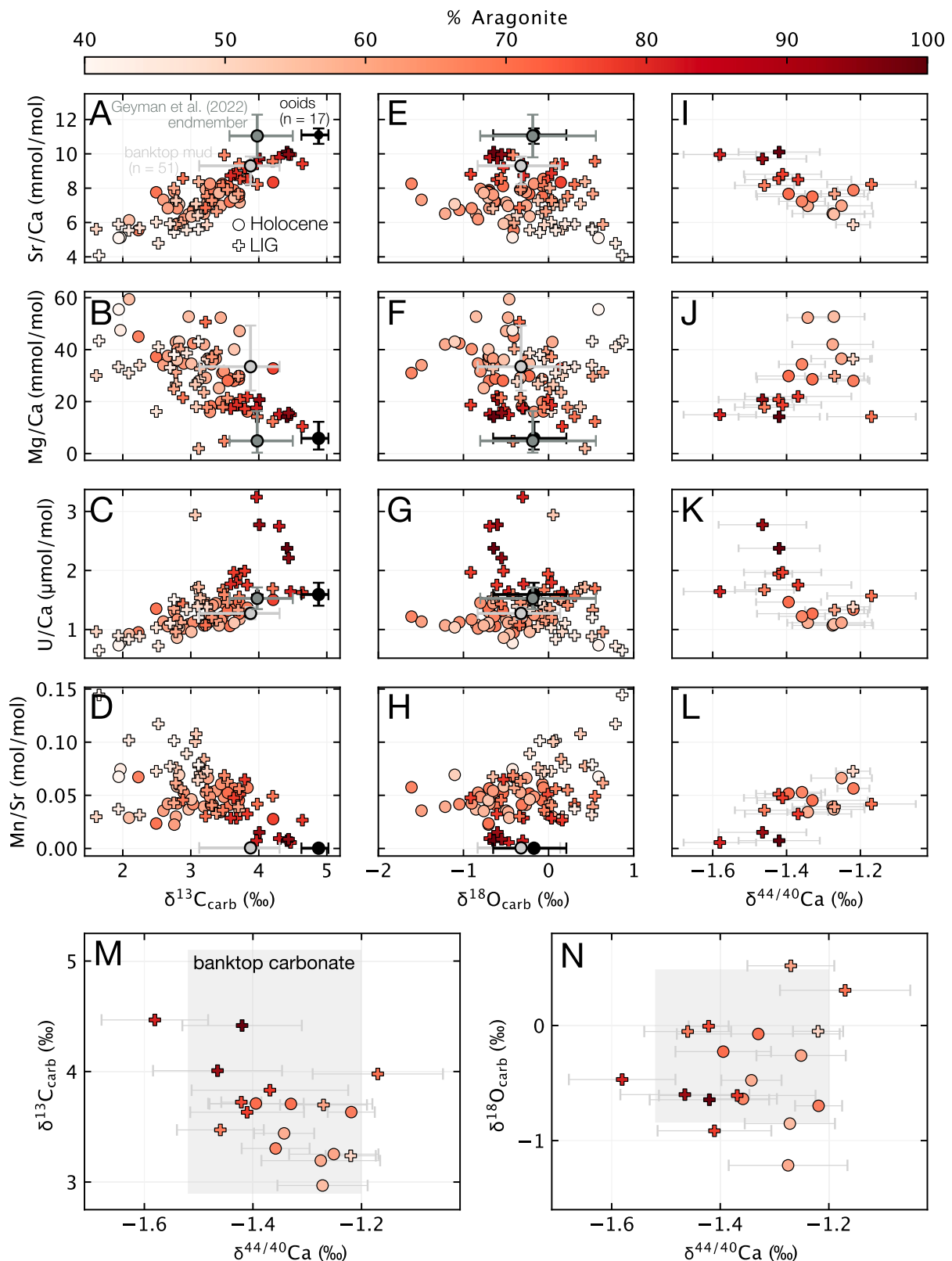
Fig. 7. We plot trace element concentrations against \delta^{13}\text{C}_{\text{carb}} (A-D), \delta^{18}\text{O}_{\text{carb}} (E-H), and \delta^{44/40}\text{Ca} (I-L). \delta^{44/40}\text{Ca} error bars are \pm 2 s.e. For comparison, we also plot the median compositions of banktop mud, ooids, and the inferred non-skeletal aragonite mud endmember from Geyman et al. (2022) with 5th and 95th percentiles. Data from glacial samples are in Figs. S6-S8. A) Interglacial Sr/Ca ranges from \sim 6 to 10 mmol/mol. B) Due to the difference in Mg concentrations between LMC ( \sim 5,000 ppm) and aragonite ( \sim 2,500 ppm), Mg/Ca decreases as \delta^{13}\text{C}_{\text{carb}} and aragonite content increase. D) Mn/Sr is low in samples with high \delta^{13}\text{C}_{\text{carb}} and aragonite content, and high in samples with low \delta^{13}\text{C}_{\text{carb}} and aragonite content. E-L) There is no apparent structure to the relationships between \delta^{18}\text{O}_{\text{carb}} or \delta^{44/40}\text{Ca} and Sr/Ca, Mg/Ca, U/Ca, or Mn/Sr during interglacials (glacial trends reflect mineralogical mixing; Fig. S6). M, N) Periplatform \delta^{44/40}\text{Ca} values for Holocene and LIG samples largely fall within the expected range for banktop carbonate, based on measurements of mud from around NW Andros Island and ooids from Joulter Cays ( -1.36 \pm 0.16\% ; Higgins et al., 2018). Banktop \delta^{13}\text{C}_{\text{carb}} and \delta^{18}\text{O}_{\text{carb}} ranges are based on the exported banktop endmember defined in Fig. 3B.
